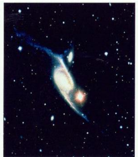
(c) NGC 6872
